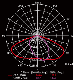
C plane lighting distributions
