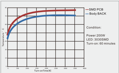
Temperature Rise
