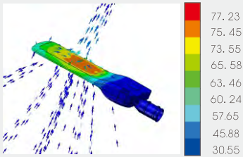
Thermal Effects to Air Unit: °C
