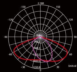
C plane lighting distributions
